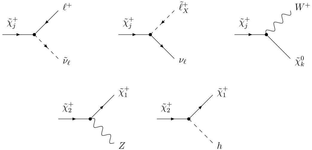
Figure 2.10: Two-body decays of charginos. Here \tilde{\ell}_X^+ = \tilde{\ell}_{L,R}^+ for \ell = e, \mu and \tilde{\ell}_X^+ = \tilde{\tau}_{1,2}^+ for \ell = \tau . The charged conjugated processes are obtained inverting the arrows and the electric charges in the Feynman diagrams.
