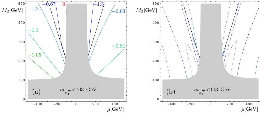
Figure 3.12: Contours of constant \gamma_{12}q_{12} (a) and \text{Im}(d_{12}^{(H)}d_{12}^{(A)*}) (b), for \tan\beta = 10 and m_A = 450 GeV. In (b) the contour lines correspond to \text{Im}(d_{12}^{(H)}d_{12}^{(A)*}) = 0.01 (dashed), 0.03 (dash-dotted) and 0.05 (dotted). The wiggly lines in both figures indicate the level crossing of the \tilde{\chi}_2^0 and \tilde{\chi}_3^0 states, with \eta_{12} = 1 in the area below and \eta_{12} = -1 in the area above the level crossing line. The gray area is experimentally excluded by m_{\tilde{\chi}_1^\pm} < 103 GeV.
