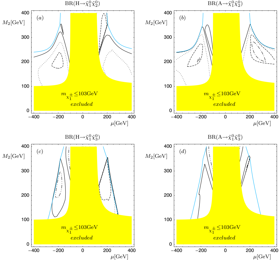
Figure 3.3: Branching ratios of the heavy Higgs bosons H and A into neutralino pairs into \tilde{\chi}_1^0 \tilde{\chi}_2^0 and \tilde{\chi}_1^0 \tilde{\chi}_3^0 for m_A = 350 GeV, \tan \beta = 5 and sfermions masses larger than M_H/2 , computed with the program HDECAY [32]. The contour lines correspond to 2 % (solid), 10 % (dotted), 20 % (dashed) and 30 % (dash-dotted). For the decays into \tilde{\chi}_1^0 \tilde{\chi}_3^0 the contour line for 5 % (dash-double-dotted) is also shown. The shaded area is the experimentally excluded region given here by m_{\tilde{\chi}_1^\pm} < 103 GeV. Also shown is the kinematical limit for the neutralino pair production processes.
