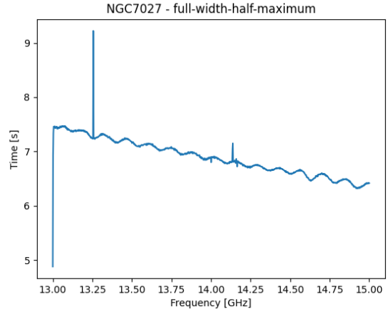
Figure 3.8: FWHM of the Gaussian fits for one scan of NGC7027. This illustrates the chance of the width of the Gaussian depending on the frequency. Outliers (at around 13, 13.3 and 14.2 GHz) are attributed to data disturbances.
