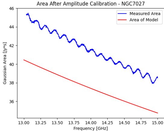
Figure 3.7: A comparison between the calibrated Area of one scan (after calibrating the amplitudes) of NGC7027 and the calculated Area of the Model is shown.
