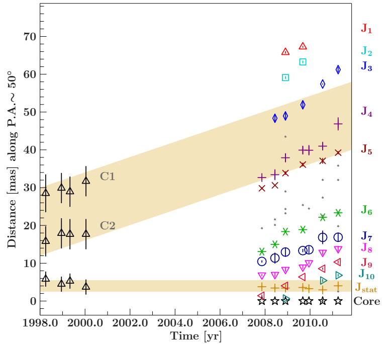
Figure 7.13: 8.4 GHz kinematic results of Cen A by Tingay et al. (2001) (open triangles) and the 2007–2011 TANAMI data. The shaded region marks the expected velocity evolution using \mu = 2 \text{ mas yr}^{-1} , which is comparable to the mean apparent speed given by the tapered TANAMI images (see text for details).
