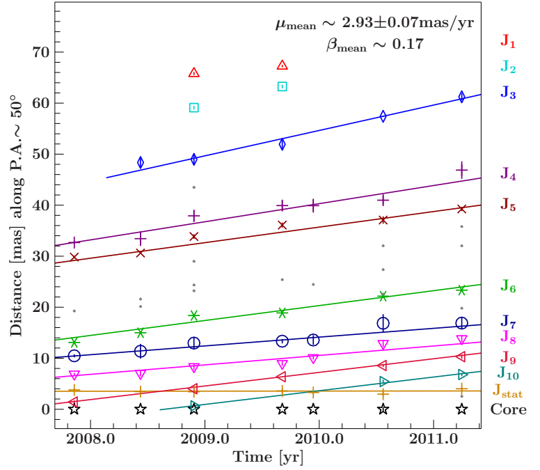
Figure 7.12: Component distance from the core component (set to zero) as a function of time. For the identified components (colored symbols), the error bars show the combination of the statistical errors and systematic errors (defined as 0.5 \times b_{\text{maj}} ) or are smaller than symbol sizes. A linear regression fit to associated components with all values weighted equally is shown. Components not included in the fit are marked in gray. Note, in particular, the components in the region of the “tuning fork” are excluded since the region is too complex. The mean apparent speed is determined for all components tracked in five or more epochs.
