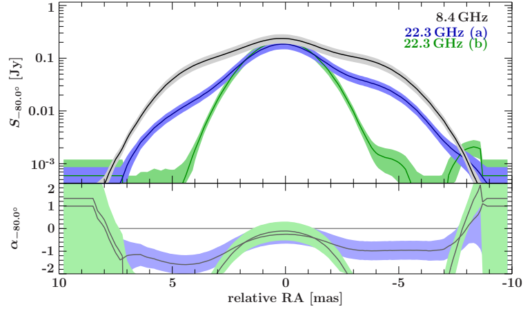
Figure 6.9: Flux density ( top ) and spectral index ( bottom ) distribution for the “blazar scenario” (see Sect. 6.4): a respective shift of \sim 2.7 mas was applied to both images in order to align the eastern component at 8.4 GHz with the brightest feature at 22.3 GHz and to get a one-sided structure with a declining spectral index distribution from “the core” downstream the jet - as expected for a blazar. This alignment leads to unphysically steep spectral indices and is therefore rejected.
