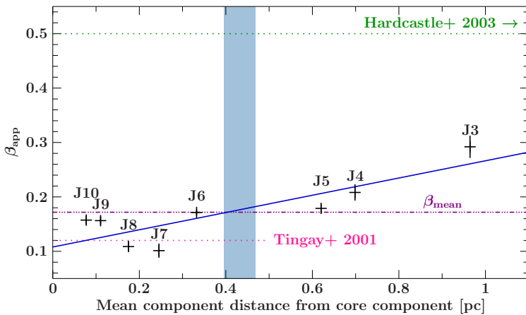
Figure 7.14: Evolution of individual component velocities as a function of mean component distance from the core component, which can be parameterized by a linear fit of \beta_{\text{app}} = 0.16d + 0.12 (blue line). The blue shaded area marks the position and extent of the jet widening (Sect. 7.6). The mean component speed and archival measurements by Tingay et al. (2001) and Hardcastle et al. (2003) are indicated by straight lines.
