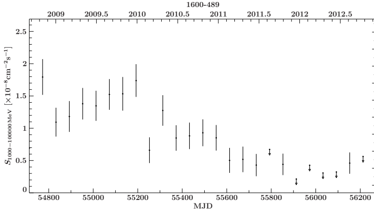
Figure 6.14: Fermi /LAT monitoring of PMN J1603–4904 over four years. Shown is the \gamma -ray light curve for the energy range 1 – 100 GeV with a binning of 60 days. Over the first two years of monitoring the source flux density showed no variability, but afterwards it constantly declined (upper limits for TS \leq 9 ).
